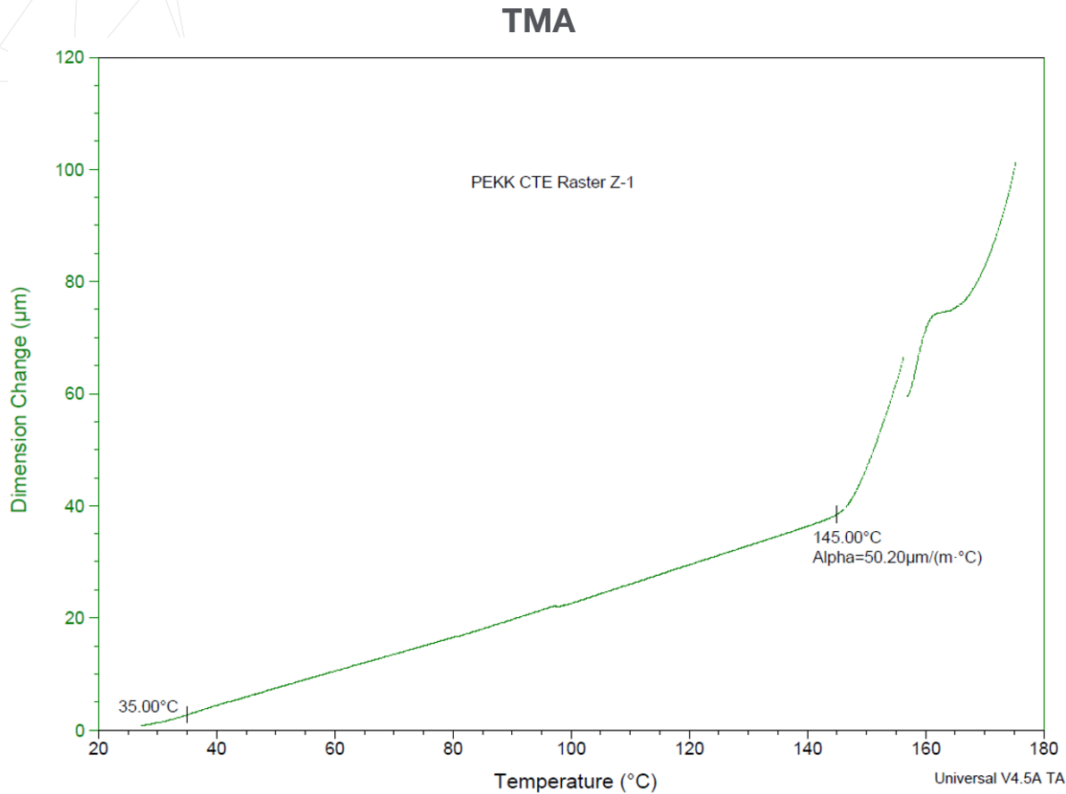
Figure 3. CTE for Antero 800NA in plane to the layers.
