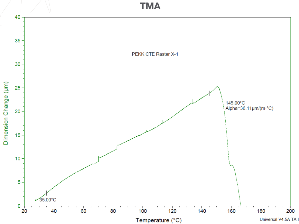
Figure 2. CTE for Antero 800NA through the layers.
