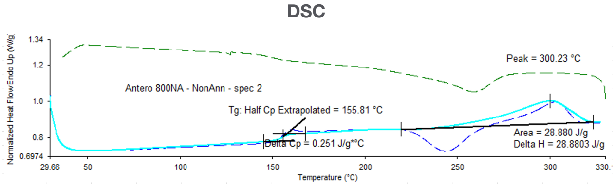
Figure 1. 2nd heating scan, DSC, for Antero 800NA.
